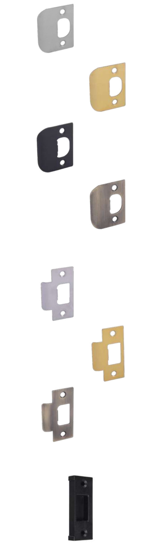
Full Lipped Strike Plate 44.4mm x 57mm x 1.2mm
